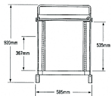
Figure 12. Agilent 1181BZ testmobile cart dimensions.
