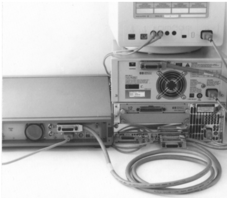
Figure 1-4 Typical GPIB connections
