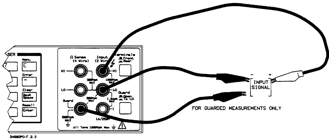
Figure 5-3 Digitizing measurement connections
