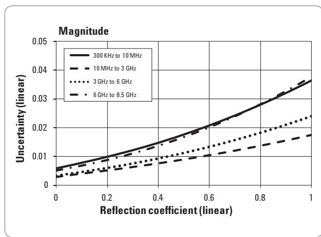
Figure 9. Reflection uncertainty (Specification)
