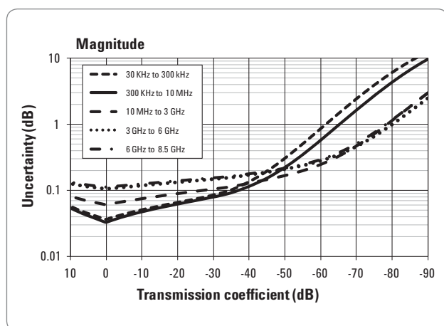
Figure 6. Transmission uncertainty (Specification)
