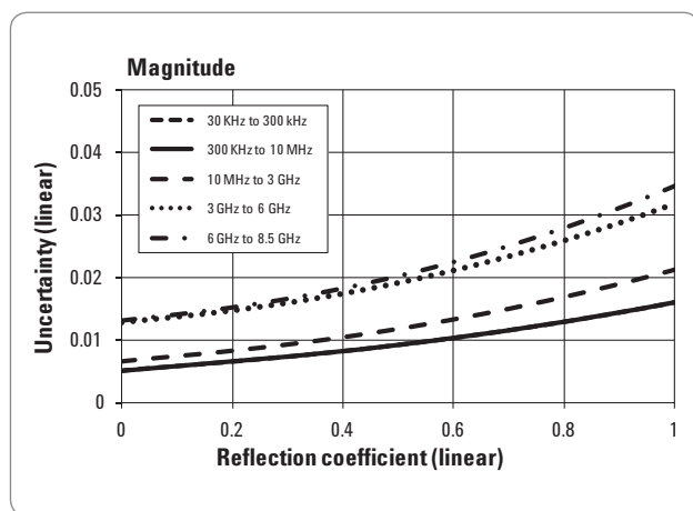
Figure 7. Reflection uncertainty (Specification)
