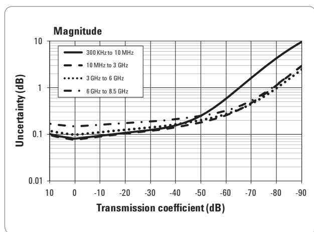
Figure 8. Transmission uncertainty (Specification)
