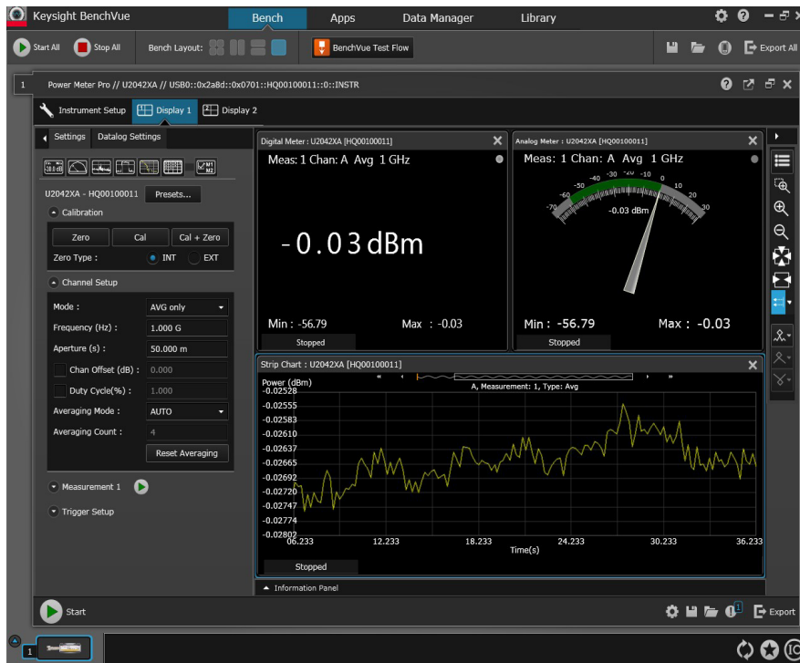
Figure 9. Digital meter, analog meter and datalog view.
