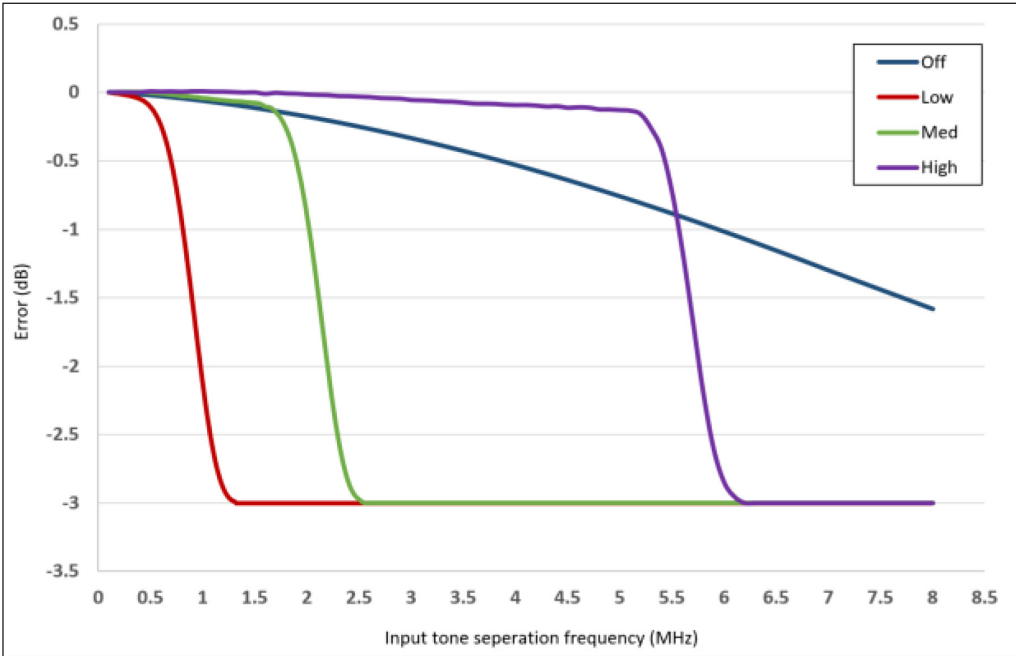
Figure 8. U2063/64/65 and L2061/62/63/64/65XA error in peak-to-average ratio measurements for a two-tone input (High, Medium, Low and Off video bandwidth settings).
