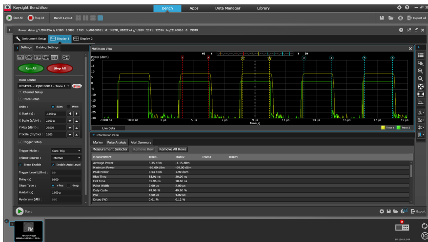
Figure 10. Multi-channel trace display with 4-pairs of gates and automatic pulse parameters measurement (sample screen shot with two U2042XAs).
