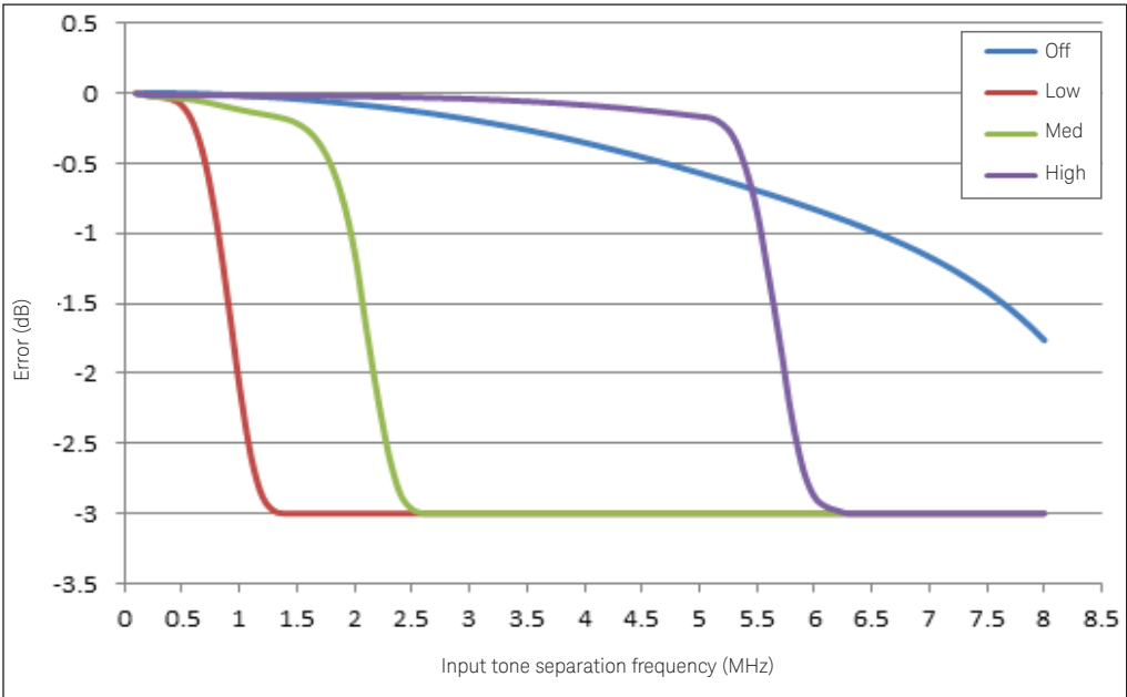
Figure 7. U2042/44/49XA and L2065XT error in peak-to-average ratio measurements for a two-tone input (High, Medium, Low and Off video bandwidth settings).
