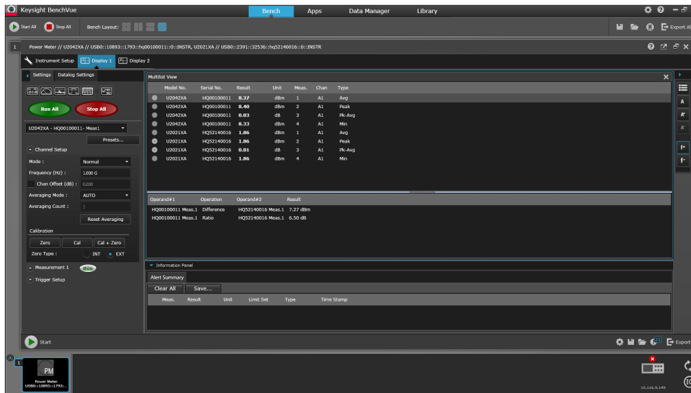
Figure 11. Multi-list view with ratio/difference function.
